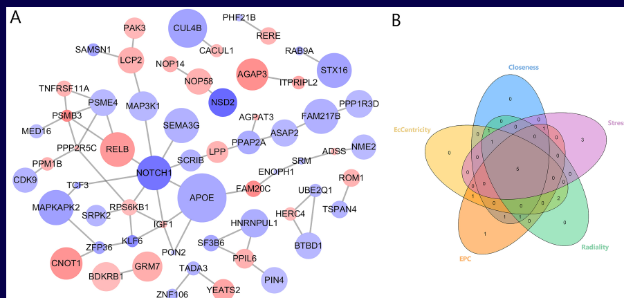
(A) PPI network of DGs. Genes with increased coverage are in red, while the blue nodes indicate the genes with decreased coverage. The darker the color of the nodes, the greater the change folds of the genes. The size of the nodes has a positive correlation with statistical significance. (B) Venn plot. We used 5 intersecting algorithms to generate a Venn plot to identify significant hub genes by employing an online analysis tool. Different algorithms are presented in different colors. The cross areas indicate the commonly accumulated DGs. Five hub genes are shown in concurrent areas (IGF1, NOTCH1, ApoE, FAM3C, and RELB). (Page 462)
